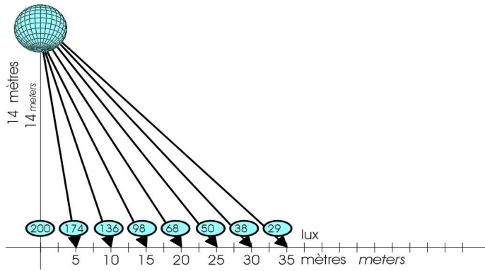
Flux lumineux Solarc 420 HMI
