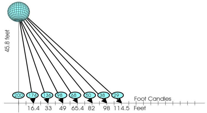
Solarc 370 HMI Lighting Chart
