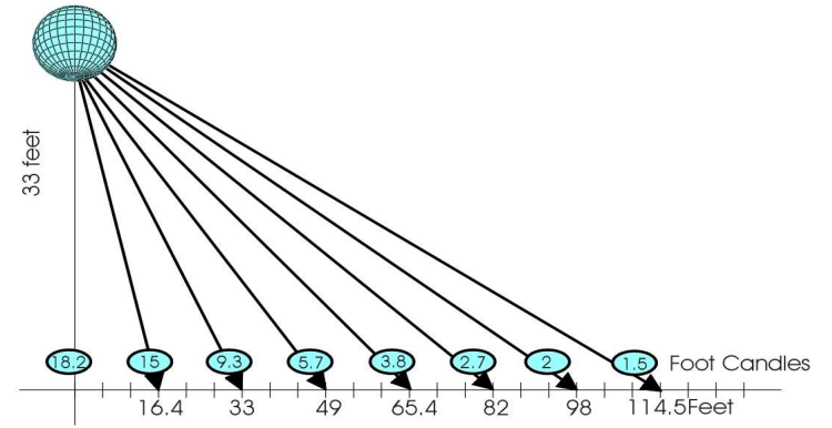
Solarc 370 HMI Lighting Chart
