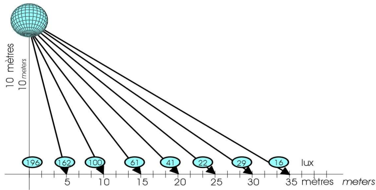
Flux lumineux Solarc 370 HMI
