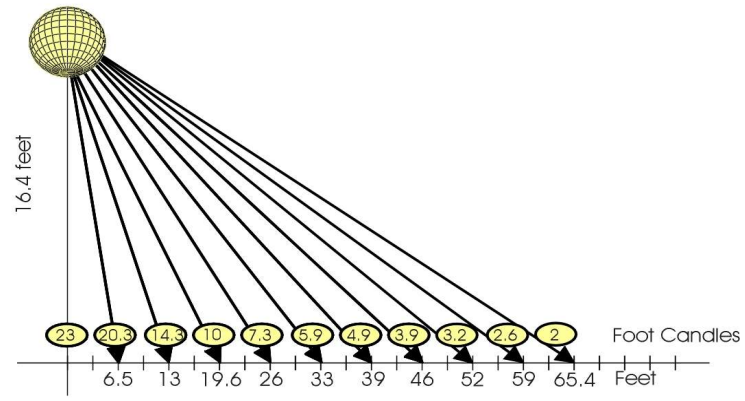
Lunix 200 Halogen Lighting Chart
