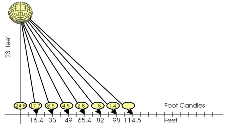
Lunix 370 Halogen Lighting Chart
